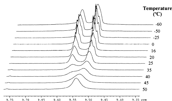
Figure 4. 1 H NMR spectrum of CHO group of compound 1 at different temperatures in CDCl 3 .
